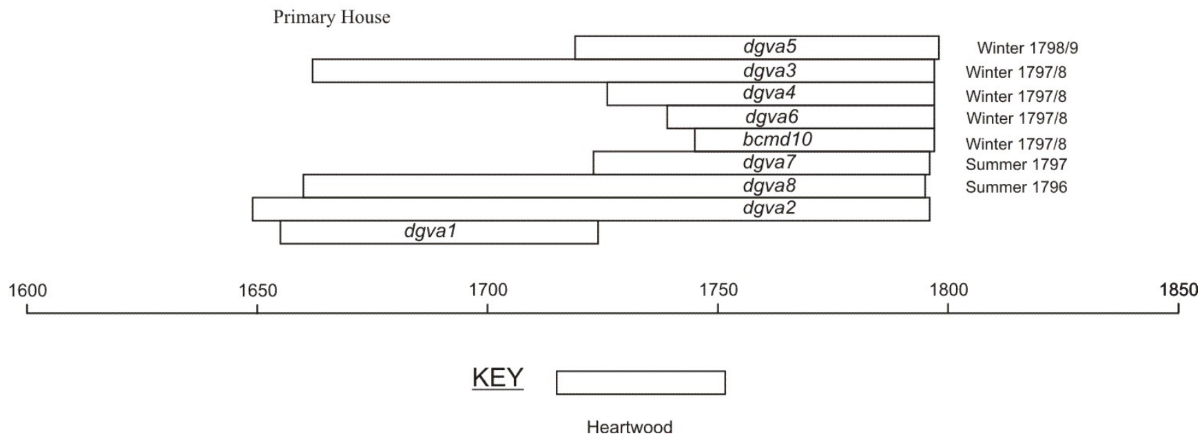
Figure 3. Bar diagram showing dated timbers in chronological order.
