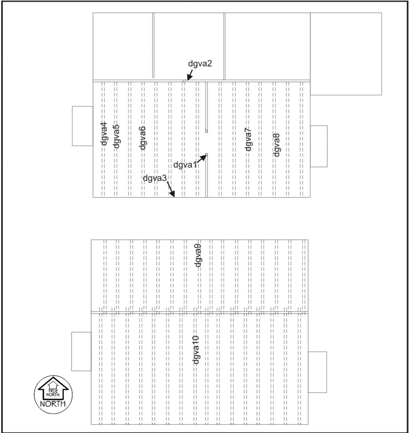
Figure 2. Sketch drawing of Edward Dromgoole House showing sample locations in the first floor (top) and second floor (bottom).
